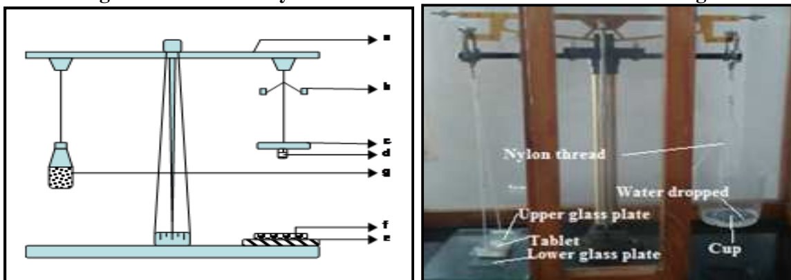
Figure No.2: detachment force measurement method
