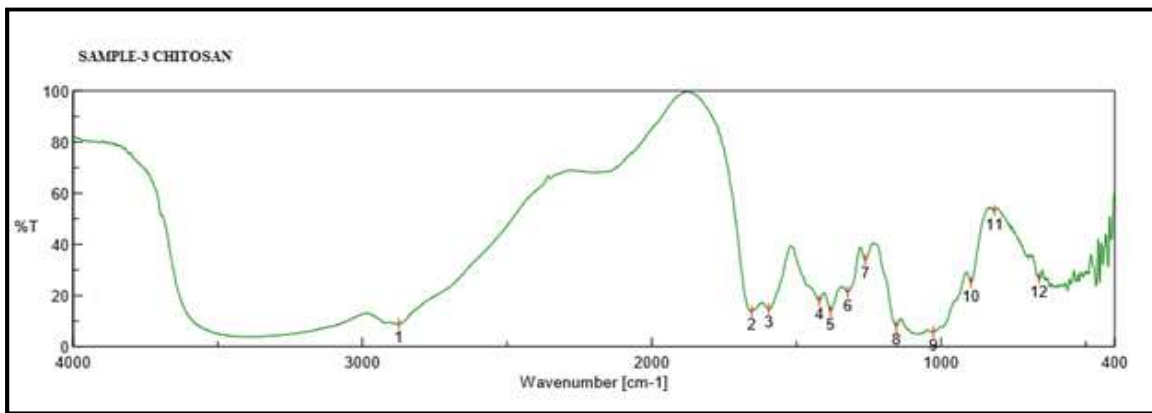
Figure No.7: FTIR spectra of Chitosan
