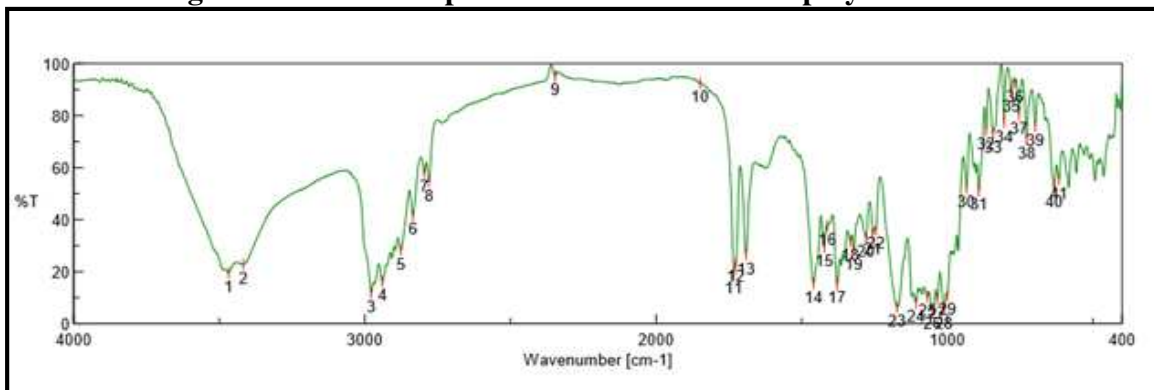
Figure No.6: FTIR spectra of Clarithromycin with Tamrarind seed polysaccharide
